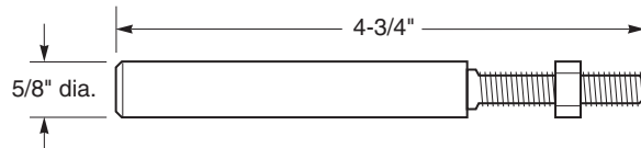
Figure-19 AM-543 Actuator Shaft Extension.
